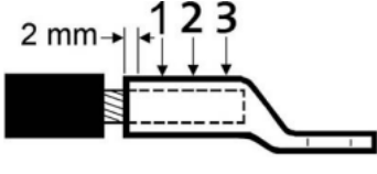
Crimp sequence for three crimps.
