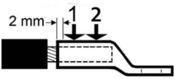
Crimp sequence for two crimps.
